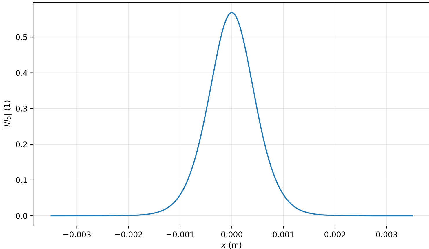
Intensity profile I(x, y = 0, z = 3.503m)/I_0 , P_{in}=0.6P_{cr} , artificial time
